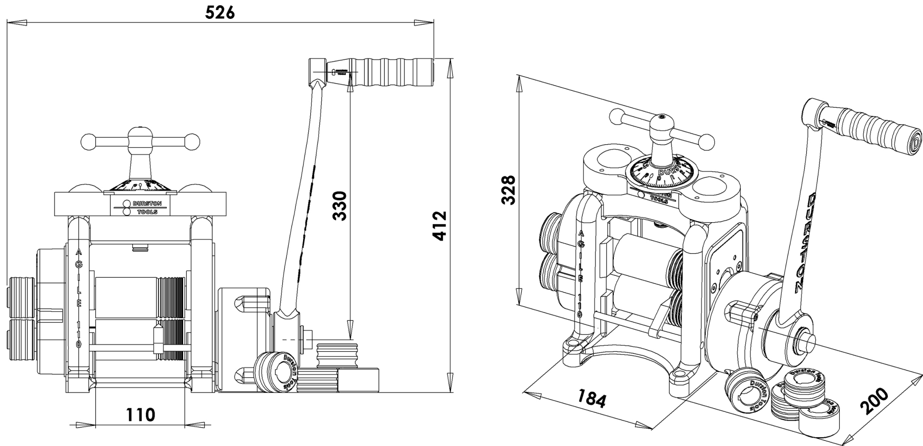
Agile Elite C110 Rolling Mill
