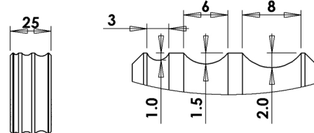
Extension Roll No2
